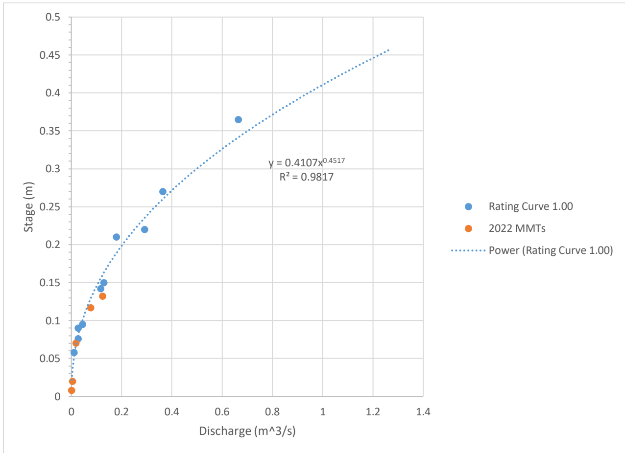
Appendix A. The rating curve model was used to estimate stream discharge in Shelly Creek during the study period.
